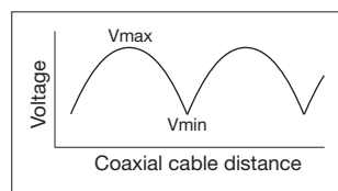
Fig. 1 Voltage Distribution Over Coaxial Cable
