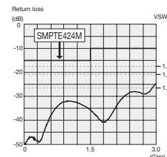
Return loss for MBCP-C3F
