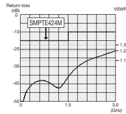
Return loss for BCJ-BPC2P
