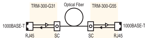
Block Diagram of TRM-300-G31 and TRM-300-G55
