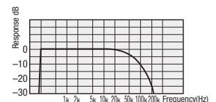
Fig. 4 Frequency Characteristics for L-4E6S (100m)
